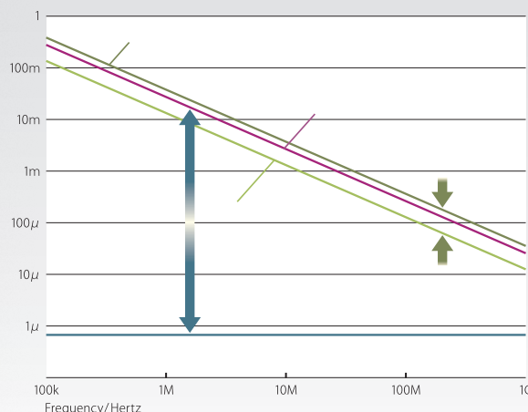
The graph below illustrates the Floating Field Damper curbing noise generated between 100kHz and 1GHz.
